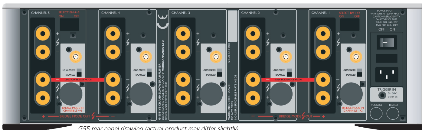
G55 rear panel drawing (actual product may differ slightly)
