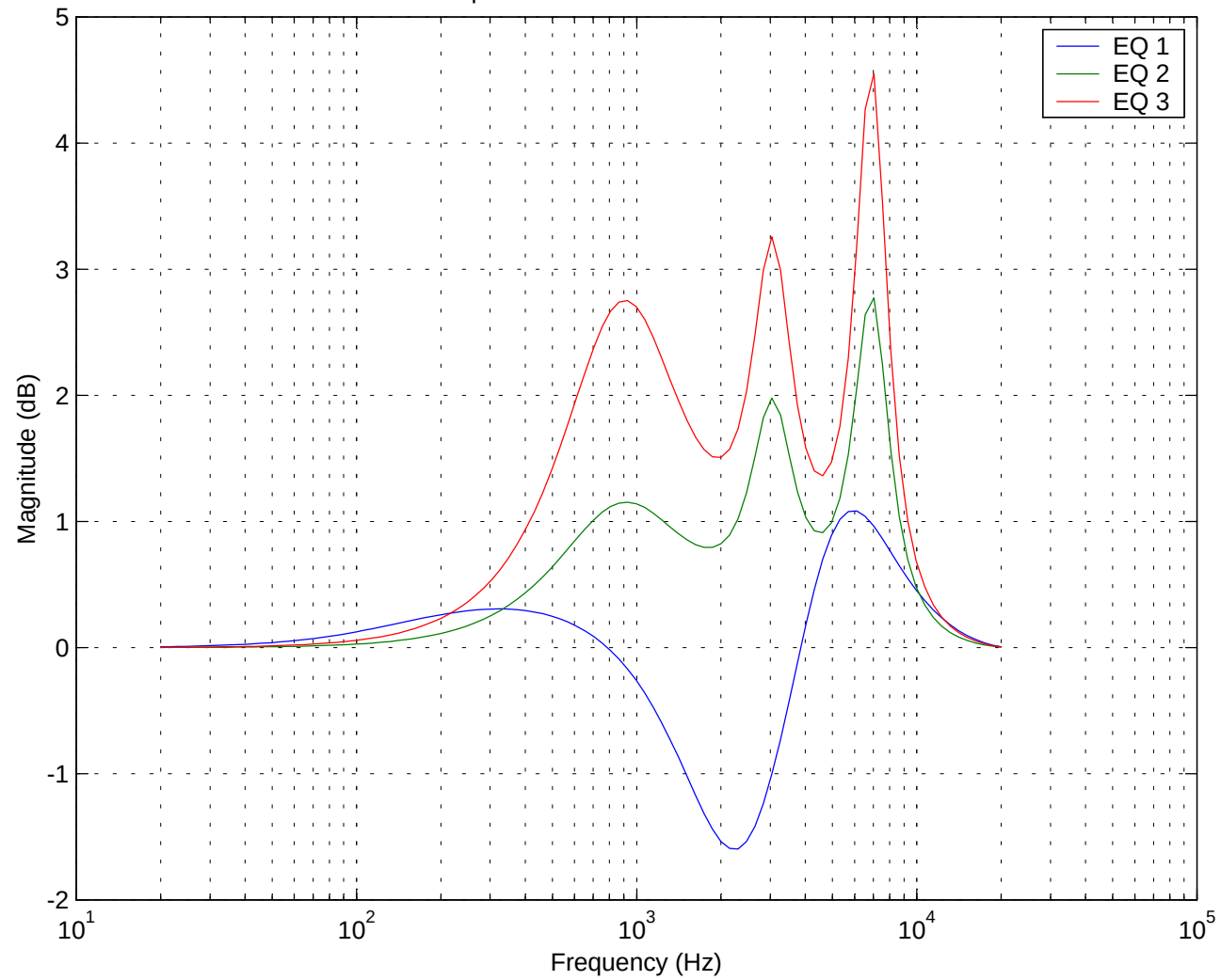
Centre Eq in Meridian Surround Sound Decoders
