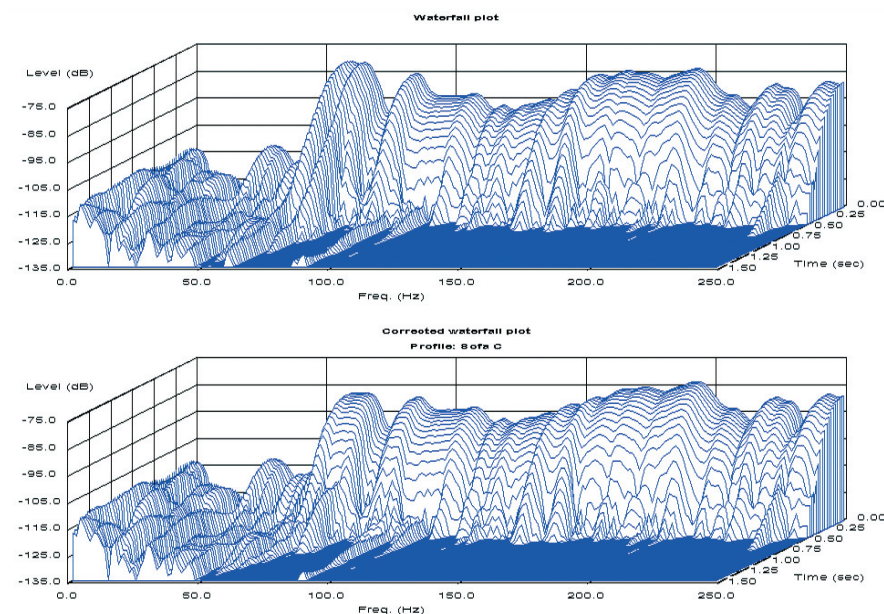
Meridian Room Correction automatically measures room nodes and computes filters to smooth out the response. It also provides 'waterfall plots' showing what the filters are doing.
